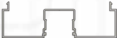
UA 7273 RECESSED MULLION CAP
