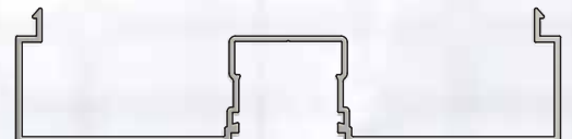
UA 7275 RECESSED MULLION CAP
