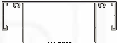
UA 7250 13mm GIB HEAD STARTER 63.5mm STUD
