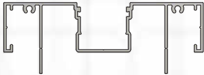
UA 7252 13mm GIB RECESSED STARTER 63.5mm STUD
